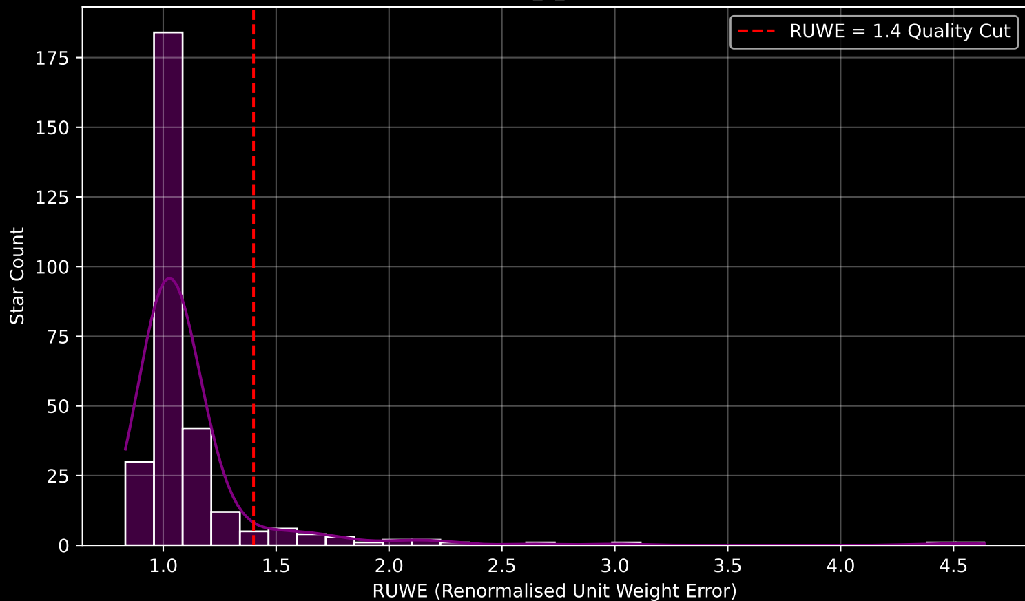
GAPOGEE DR17 Field [CygnusX_C_btx] RUWE Distribution (n= 296)
