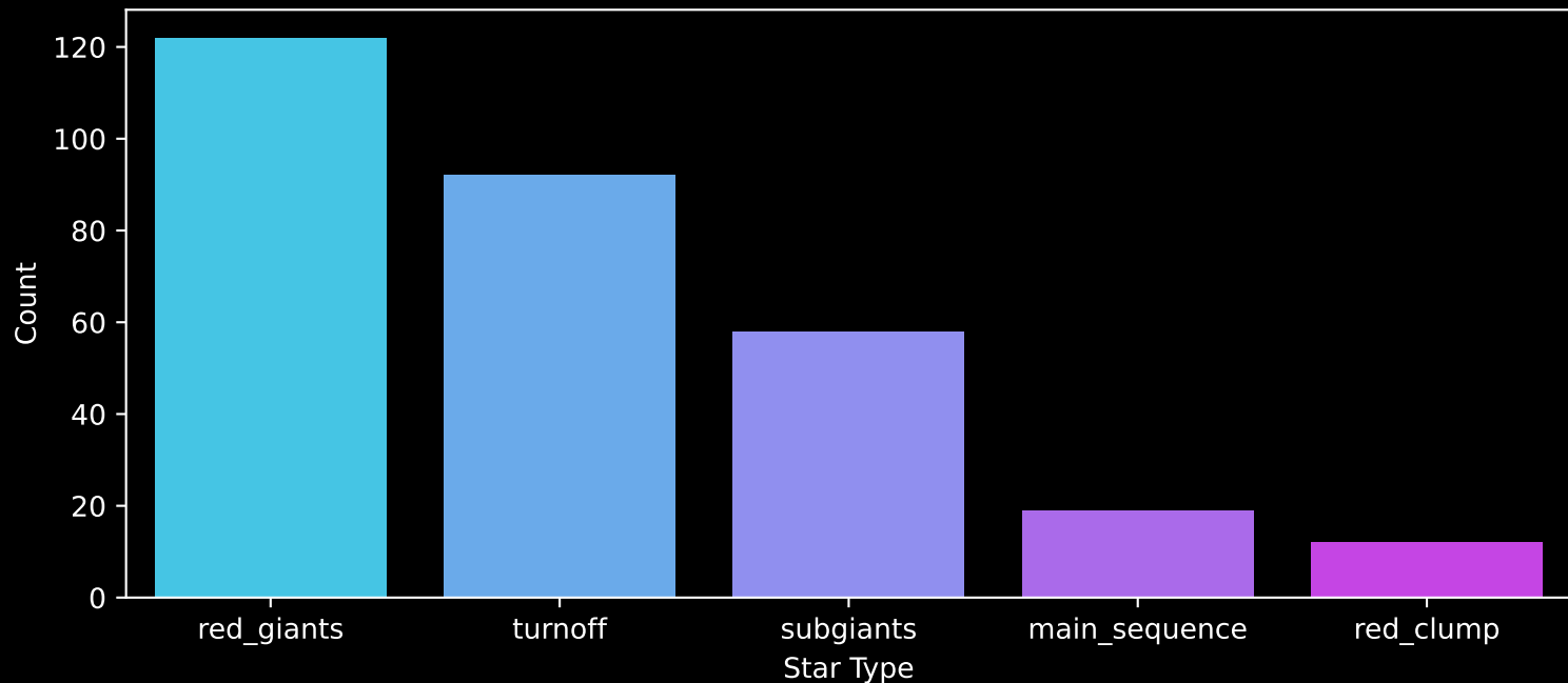
APOGEE DR17 Field: [CygnusX_C_btx] Count plot of Star Type
