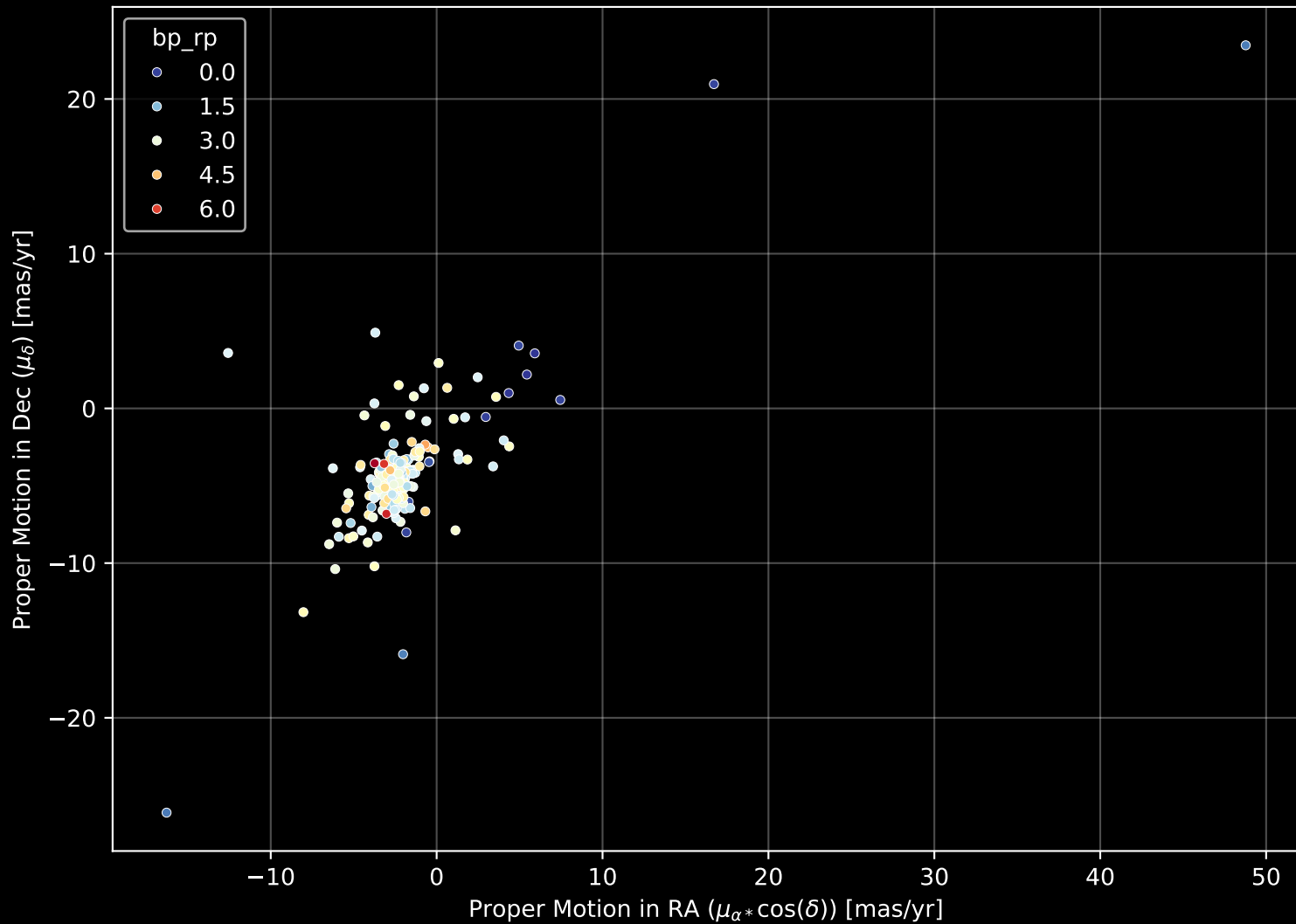
APOGEE DR17 Field: [CygnusX_C_btx] Proper Motion Diagram (n= 303)
