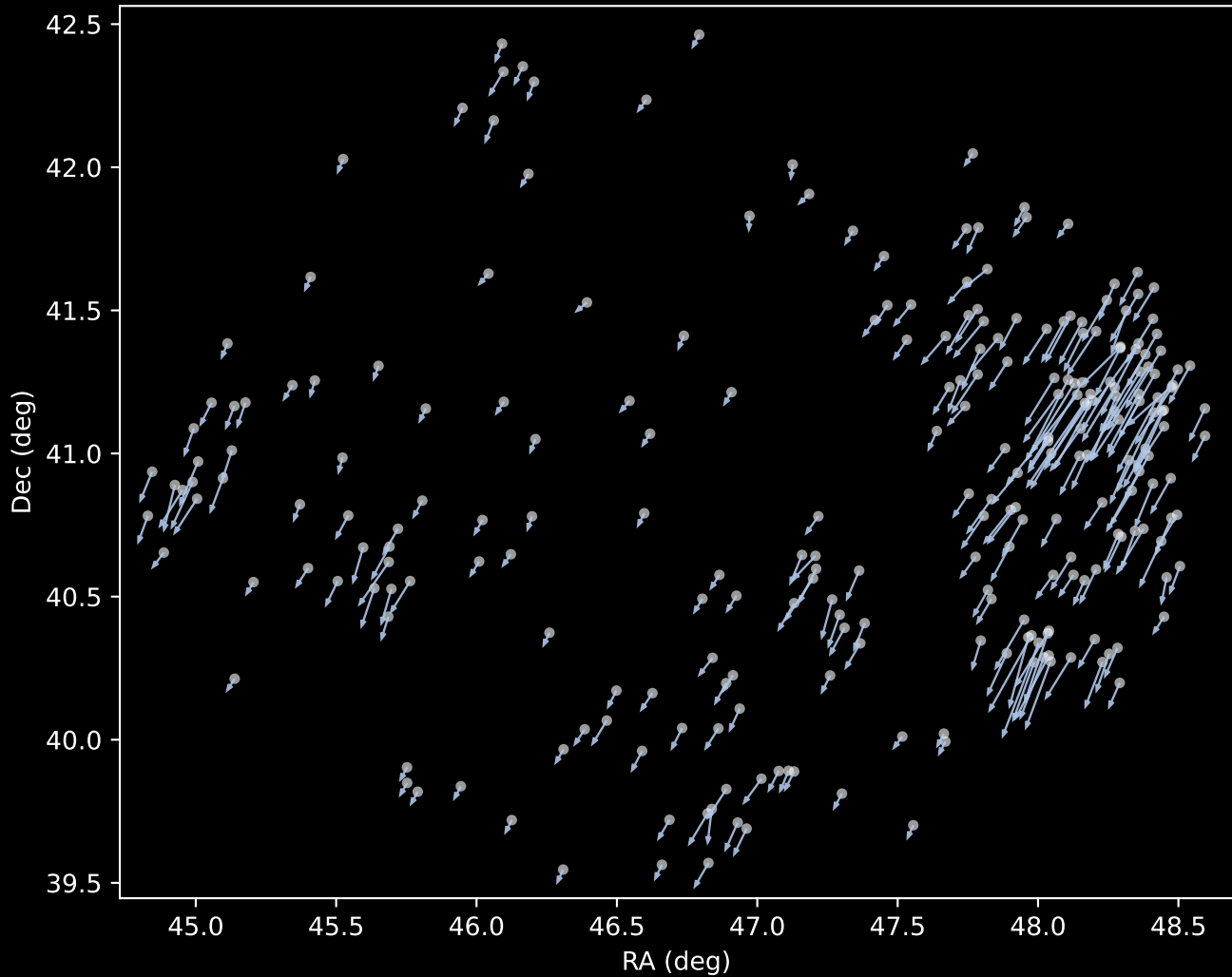
APOGEE DR17 Cluster 1 Proper Motion Vectors (n=252)
