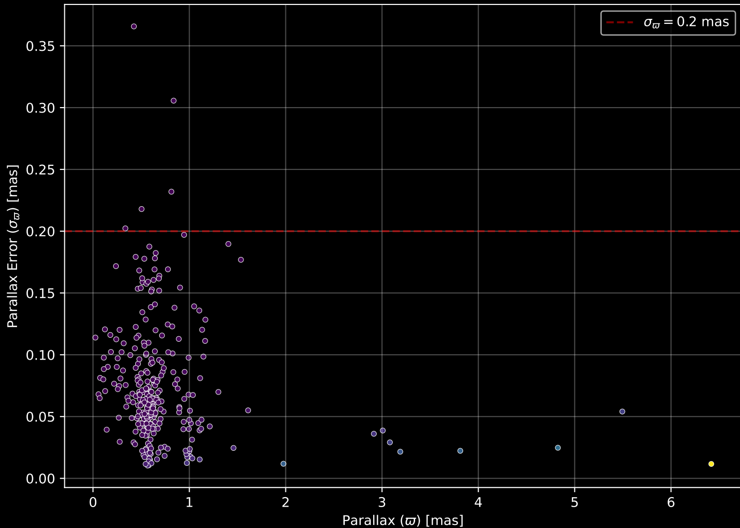
APOGEE DR17 Field: [CygnusX_C_btx] Parallax Quality (n= 303)
