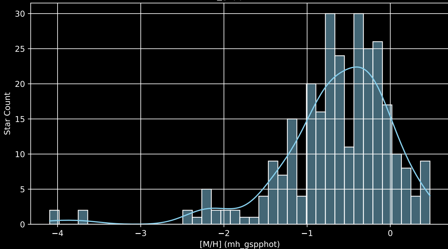
APOGEE DR17 Field: [CygnusX_C_btx [M/H] (mh_gspphot) (n= 289)
